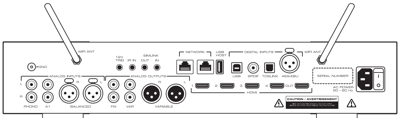
Figure 2: 390 Backpanel
