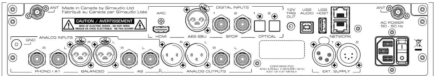
Drawing 2: rear panel
